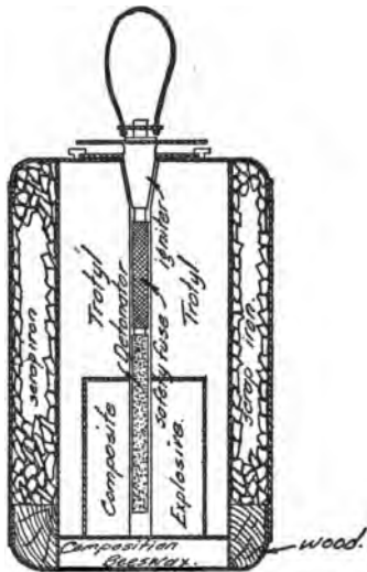
SECTION. Dimension of Cylinder 4 x 2 1/2" HAND GRENADE NO. 7.
